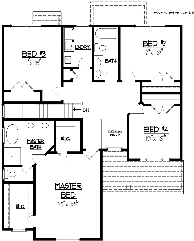
SECOND FLOOR PLAN 1,130 SQ. FT.
