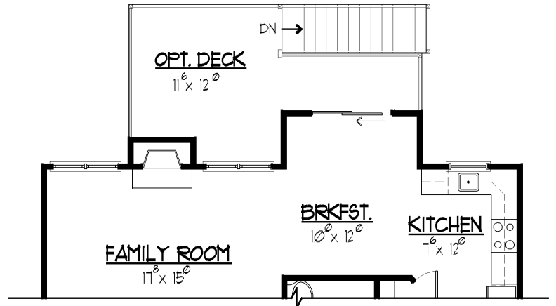
PARTIAL FIRST FLOOR PLAN w/ BRKFST. OPTION 824 SQ. FT.
